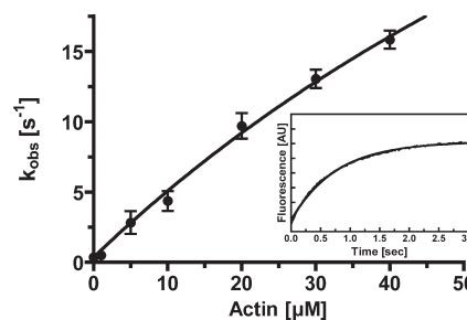
FIGURE 6: Release of phosphate from acto-p-huM3AMD. The rate of release of phosphate from huM3AMD was measured by using MDCC-PBP. p-huM3AMD (1.5 \mu\text{M} ) was mixed with 60 \mu\text{M} MgATP, aged for 5 s, and then mixed with 3 \mu\text{M} phosphate binding protein in the presence and absence of actin. The actin concentration dependence of the rate of phosphate release is shown. The apparent rate was increased with actin concentration to yield the maximum rate of phosphate release of 70 \pm 24 \text{s}^{-1} and a K_{\text{actin}} of 138 \pm 58 \mu\text{M} . The error bars represent the standard error from three to six independent experiments. The inset shows a typical recording of the MDCC-PBP fluorescence change at 5 \mu\text{M} F-actin. Time course fits to double-exponential kinetics with a fast k_{\text{obs}} of 2.0 \text{s}^{-1} .
