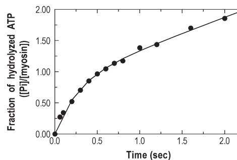
FIGURE 5: P i burst of p-huM3MD. The quenched-flow experiment was conducted after 1.4 \mu\text{M} p-huM3AMD and 30 \mu\text{M} [ \gamma - 32 P]ATP were mixed and allowed to age for the indicated time. The solid line is the best fit to an initial single-exponential P i liberation followed by the steady-state rate. The observed P i burst size and the initial hydrolysis rate are 0.84 and 3.7 \text{s}^{-1} , respectively.
